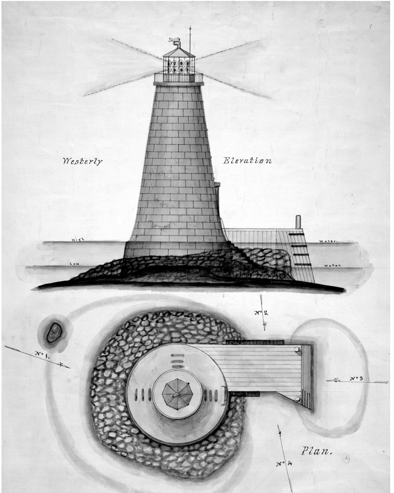
Elevation and plan of Execution Rocks Lighthouse, New York, 1849
