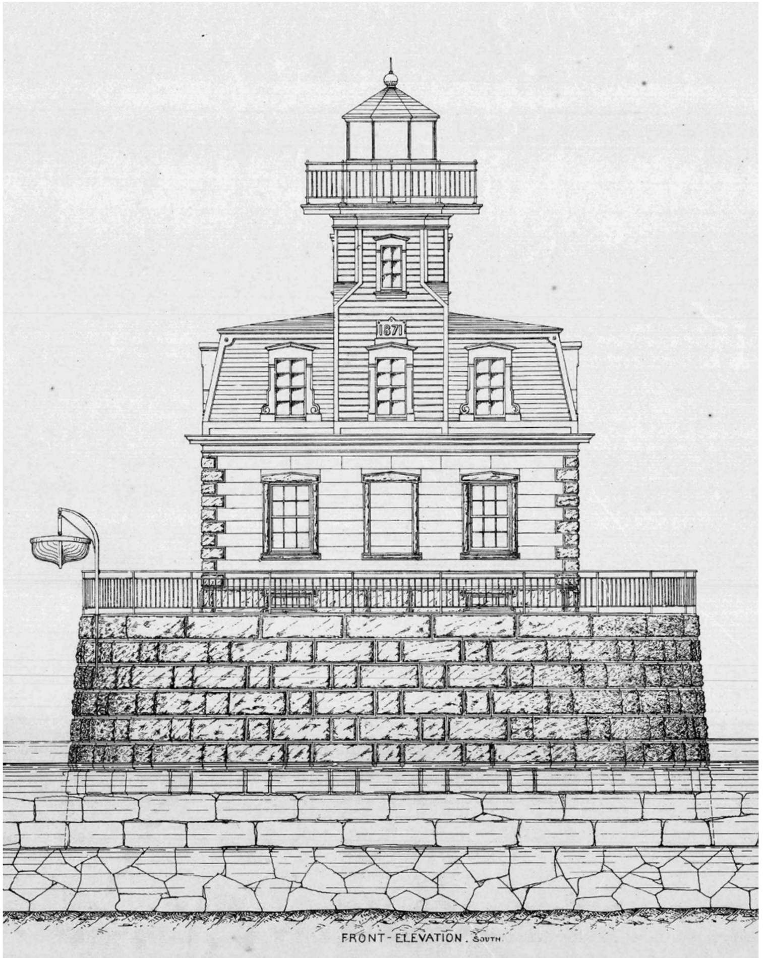
Elevation of Penfield's Lighthouse, Connecticut, 1870
