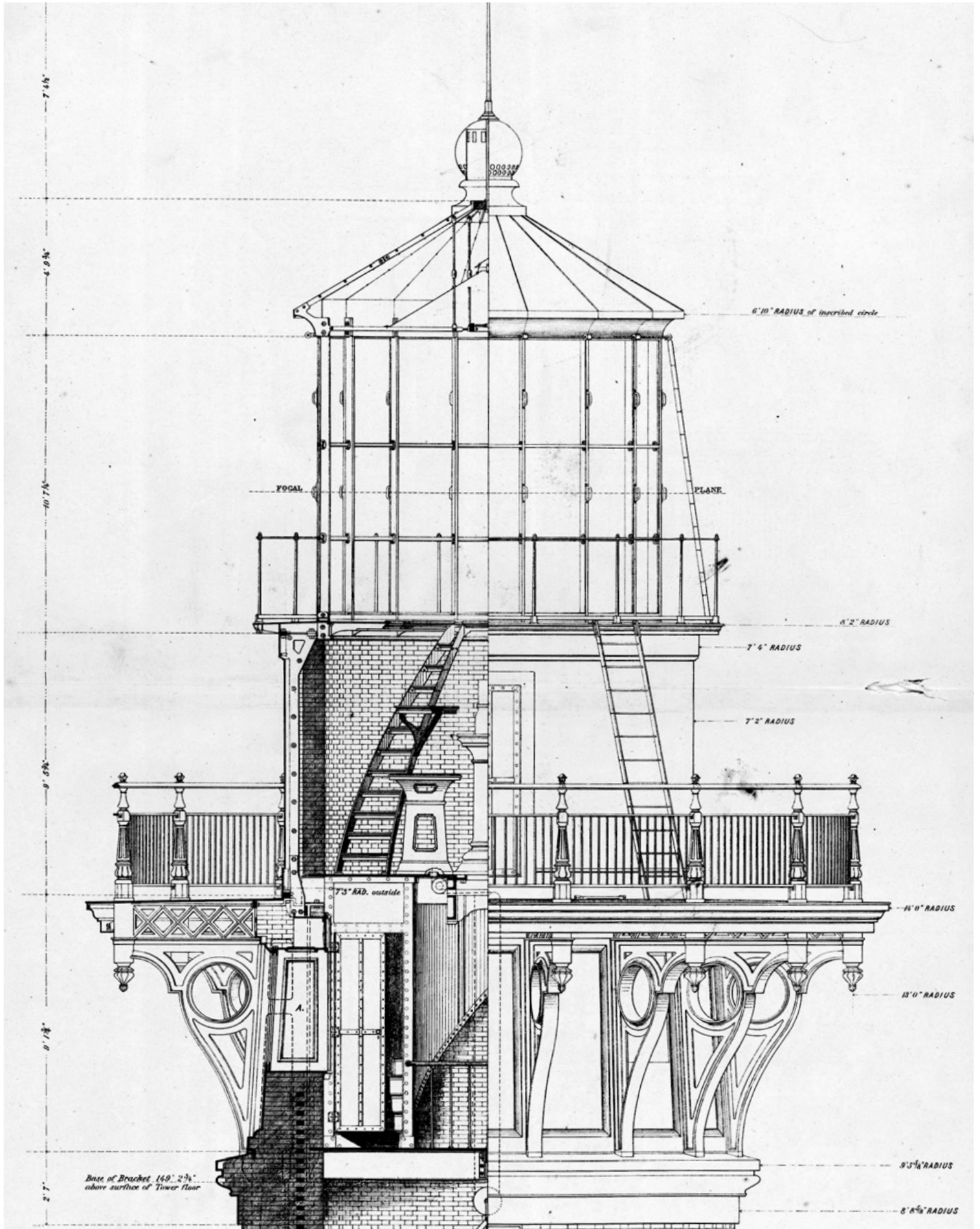
Drawing showing the upper part of the lantern tower for the lighthouse at Cape Hatteras, North Carolina, 1869
