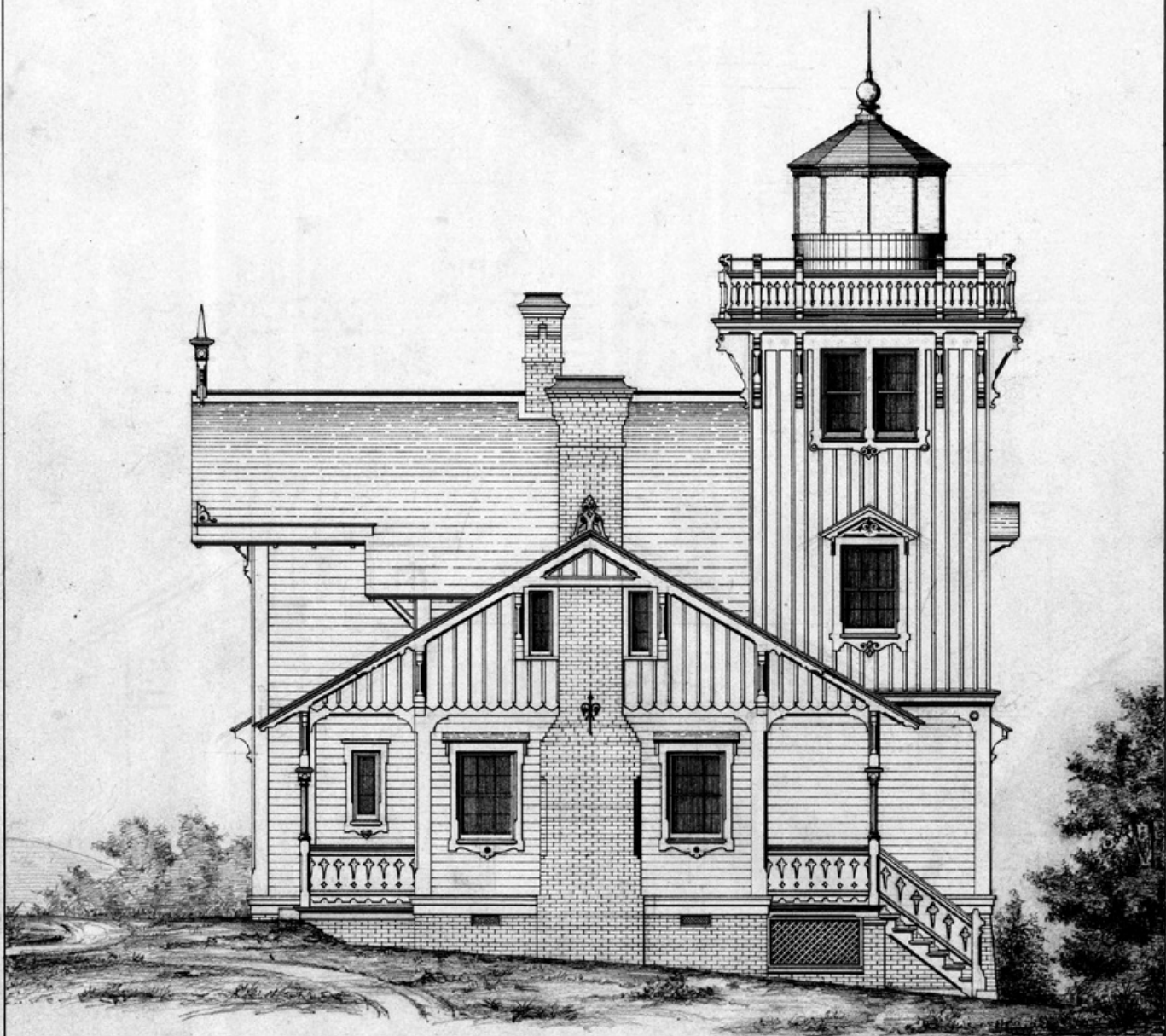
NORTH ELEVATION
