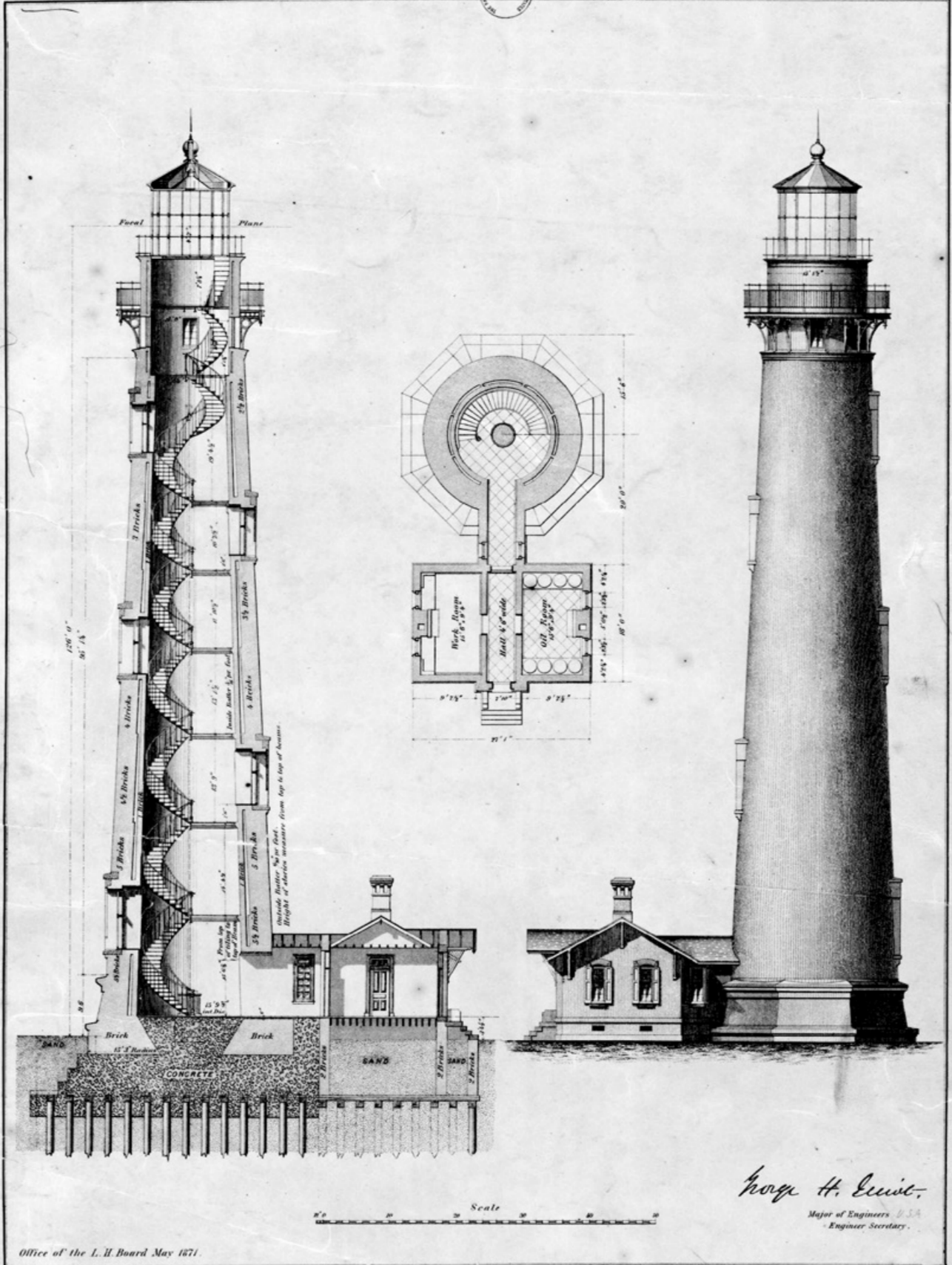
Section, elevation, and plan drawing for the lighthouse at Sand Island, Alabama, 1871
