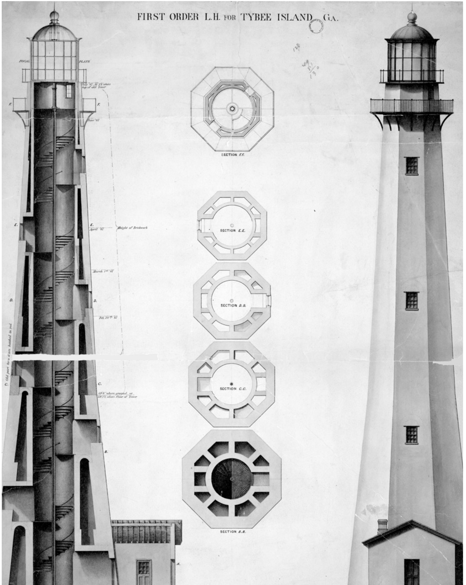
Elevation, section, and plan of a first order lighthouse at Tybee Island, Georgia, 1867
